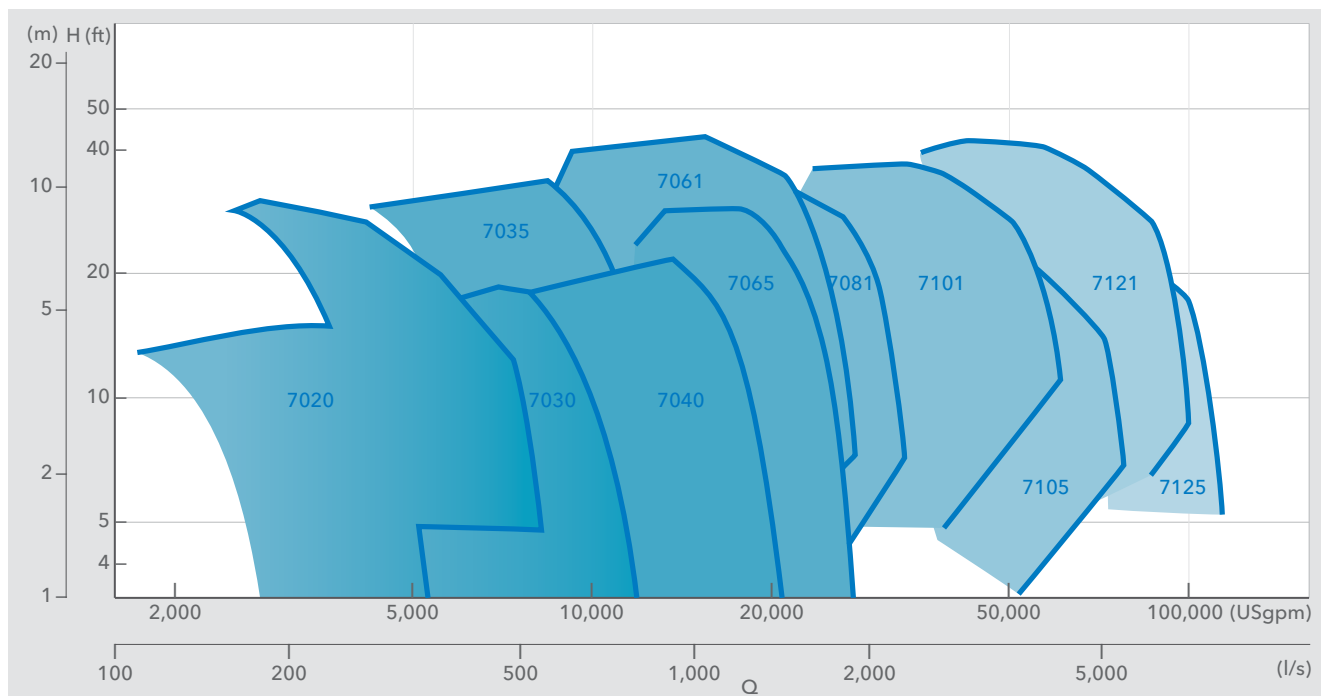
Performance 60 Hz
